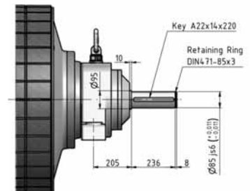
Standard External Brake Shaft Dimension
