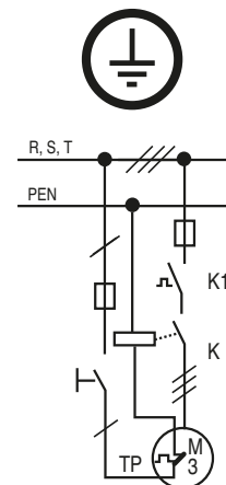
Earth connection
