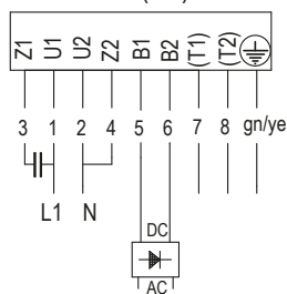
1-Ph-Motor (EB)
