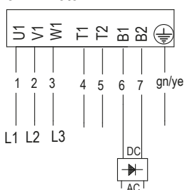
3-Ph-Motor EB
