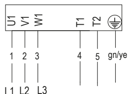
3-Ph-Motor
