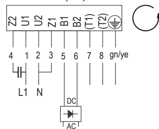
1-Ph-Motor (EB)
